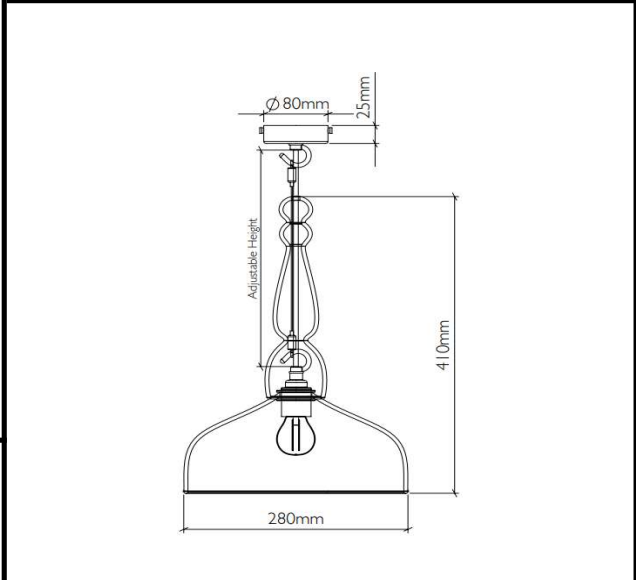
Dimension diagram
